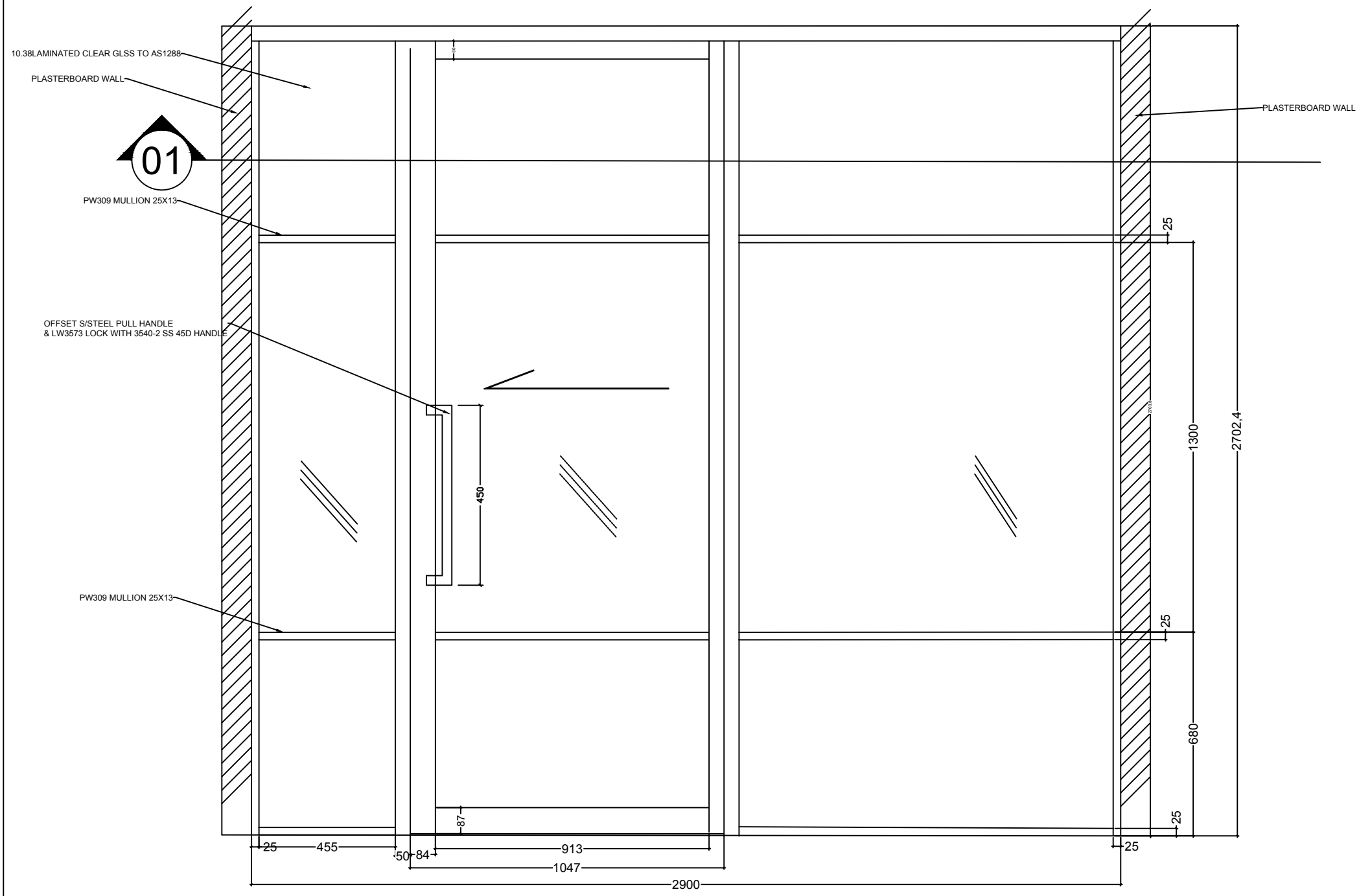
01 FRONT ELEVATION PS02 LEFT HAND ENTRY
