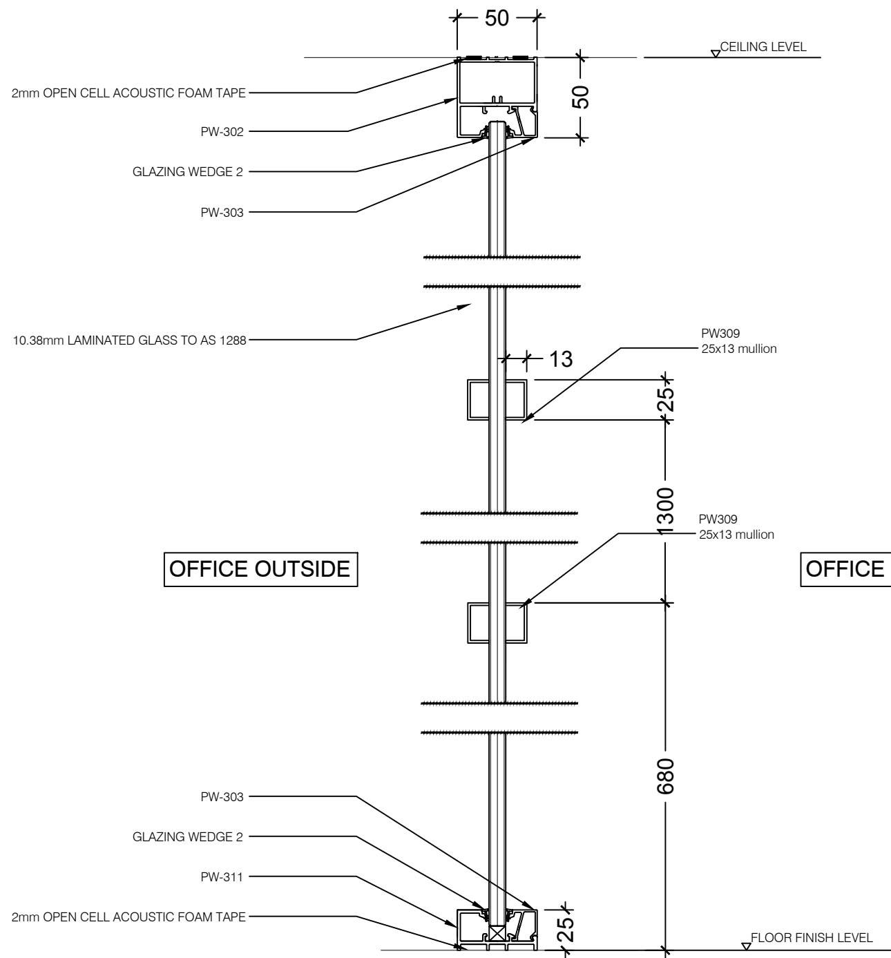
A VERTICAL SECTION X SINGLE GLAZING
